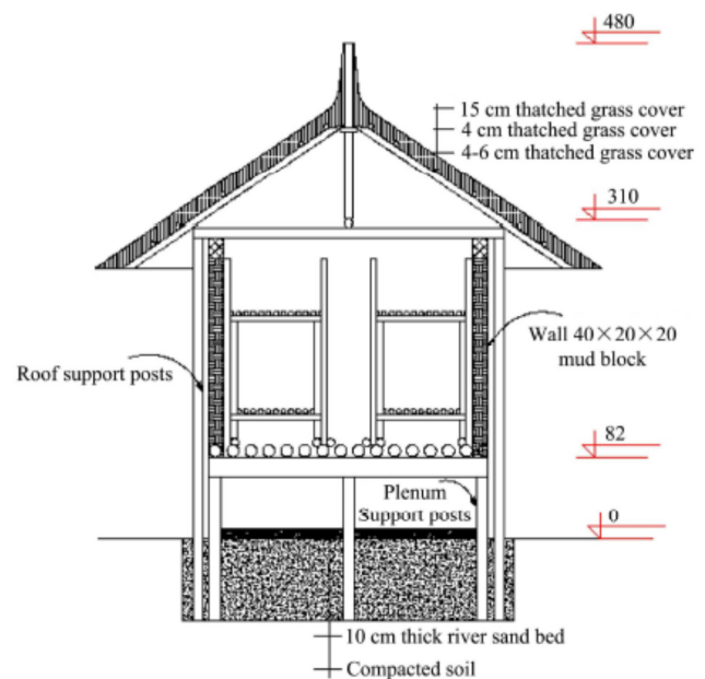
Figure 2. Naturally ventilated potato store.
